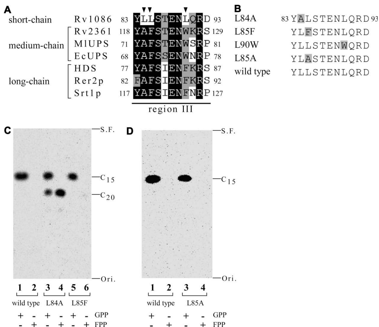
Fig. 1. Introduction of mutations in Rv1086. (A) Alignment of amino acid sequences around conserved regions III and V of various cis -prenyltransferases: Rv1086, E,Z -FPP synthase from M. tuberculosis (Accession No. D70895); Rv2361c, decaprenyl diphosphate synthase from M. tuberculosis (H70585); MIUPS, UPS from M. luteus B-P 26 (BAA31993); EcUPS, UPS from E. coli (Q47675); Rer2p, dehydrolidichyl diphosphate (DedolPP) synthase from S. cerevisiae (BAA36577); Srt1p, DedolPP synthase from S. cerevisiae (NP_013819); and HDS, DedolPP synthases from human (BAC57588). The sequences were aligned using CLUSTAL W program [20]. Identical residues (five or more) are shown in black, and similar residues are shaded. The arrowheads indicate the characteristic amino acid residues of Rv1086. (B) Partial amino acid sequences around region III of wild type and mutant enzymes are aligned. The substituted amino acid residues are shaded. (C) TLC autoradiogram of the reaction products of wild type and mutant enzymes. Lanes 1 and 2, wild type; lanes 3 and 4, L84A; lanes 5 and 6, L85F. The products were analyzed as described in Materials and methods. Each reaction mixture contained 10 \mu\text{M} GPP (lanes 1, 3 and 5) or E,E -FPP (lanes 2, 4 and 6) as an allylic substrate. Under all assay conditions, less than 30% of each substrate reacted. Ori., origin; S.F., solvent front. (D) TLC autoradiogram of the reaction products of wild type and L85A. Lanes 1 and 2, wild type; lanes 3 and 4, L85A. The products were analyzed as described in Materials and methods. Each reaction mixture contained 10 \mu\text{M} GPP (lanes 1 and 3) or E,E -FPP (lanes 2 and 4) as an allylic substrate. Under all assay conditions, less than 30% of each substrate reacted. Ori., origin; S.F., solvent front.
