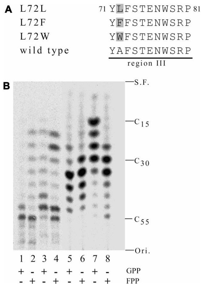
Fig. 2. Introduction of substitution mutations into region III of UPS from M. luteus B-P 26. (A) Partial amino acid sequences around region III of wild type and mutant enzymes are aligned. The substituted amino acid residues are shaded. (B) TLC autoradiogram of the reaction products of wild type and mutant enzymes. Lanes 1 and 2, wild type; lanes 3 and 4, A72L; lanes 5 and 6, A72F; and lanes 7 and 8, A72W. The products were analyzed as described in Materials and methods. Each reaction mixture contained 10 μM GPP (lanes 1, 3, 5, and 7) or E,E -FPP (lanes 2, 4, 6, and 8) as an allylic substrate. Under all assay conditions, less than 30% of each substrate reacted. Ori., origin; S.F., solvent front.
