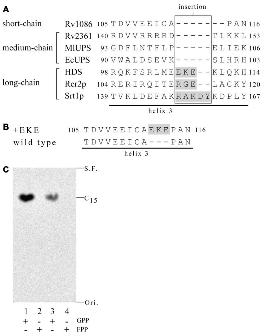
Fig. 3. Introduction of extra amino acid insertions into helix-3 of Rv1086. (A) Alignment of amino acid sequences around helix-3 of various cis -prenyltransferases. Similar notations as those in Fig. 1 are used for sequences. The extra amino acid insertions that are characteristic for long-chain cis -prenyltransferase are shaded. (B) Partial amino acid sequences around helix-3 of Rv1086 and mutant enzymes are aligned. The introduced extra amino acid insertions are shaded. (C) TLC autoradiochromatogram of the reaction products of wild type and mutant enzymes. Lanes 1 and 2, wild type and lanes 3 and 4, +EKE. The products were analyzed as described in Materials and methods. Each reaction mixture contained 10 \mu M GPP (lanes 1 and 3) or E,E -FPP (lanes 2 and 4) as an allylic substrate. Under all assay conditions, less than 30% of each substrate reacted. Ori., origin; S.F., solvent front.
